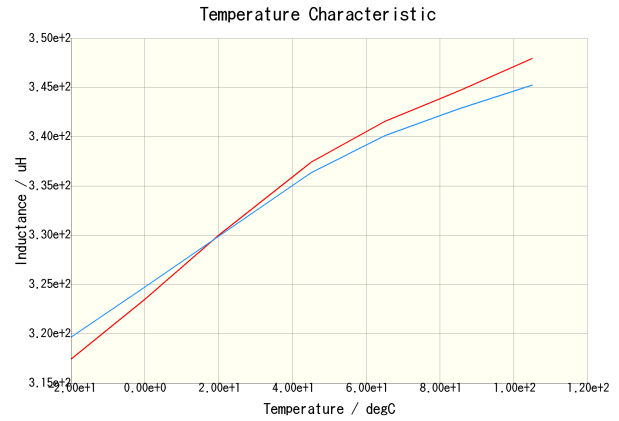
CLF7045T-331M(DC = 0A)
