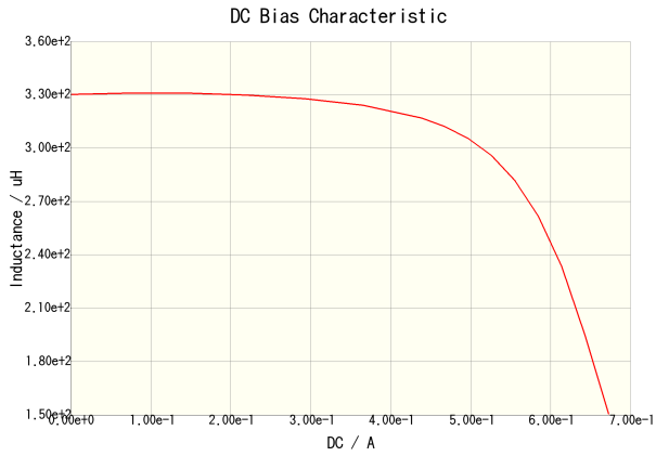
CLF7045T-331M(Amb. Temp. = 20degc)
