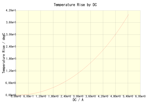
CLF10040T-3R3N(Amb. Temp. = 20degc)
