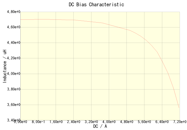
CLF10040T-4R7N(Amb. Temp. = 20degc)
