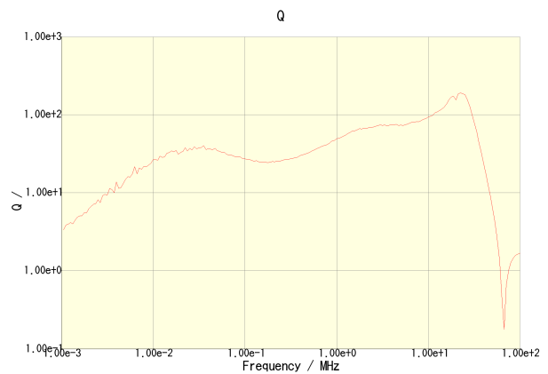
CLF10040T-4R7N
