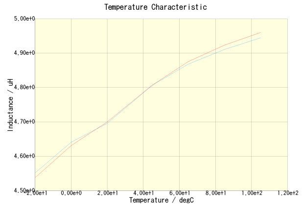
CLF10040T-4R7N(DC = 0A)
