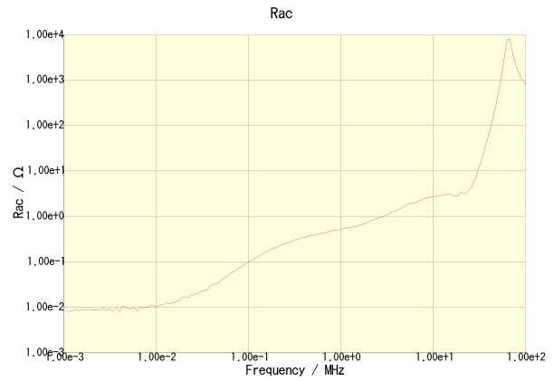
CLF10040T-4R7N
