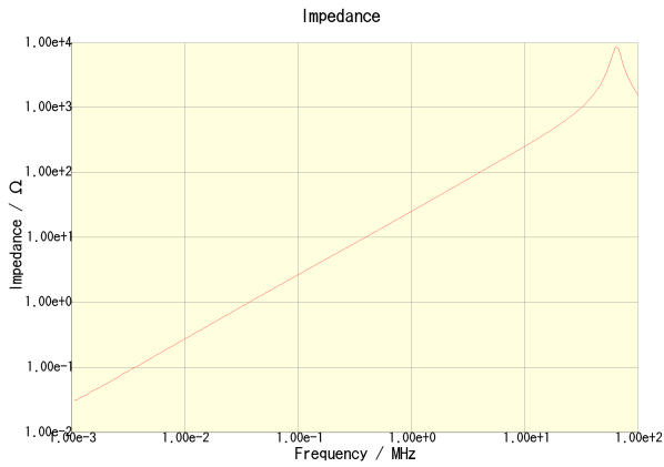
CLF10040T-4R7N
