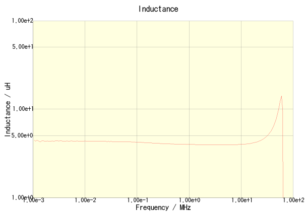
CLF10040T-4R7N
