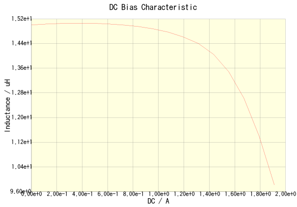
CLF6045T-150M(Amb. Temp. = 20degc)
