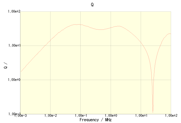
CLF6045T-150M
