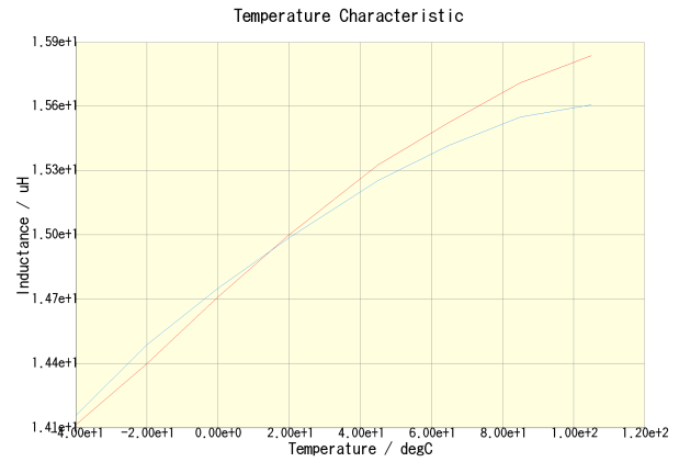
CLF6045T-150M(DC = 0A)
