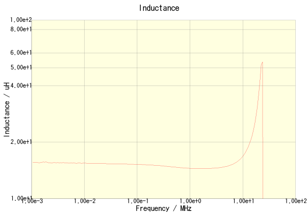
CLF6045T-150M
