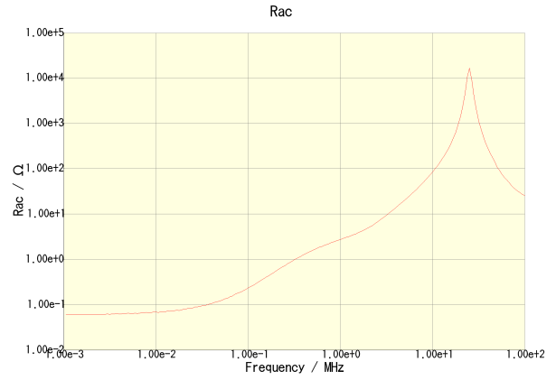
CLF6045T-150M
