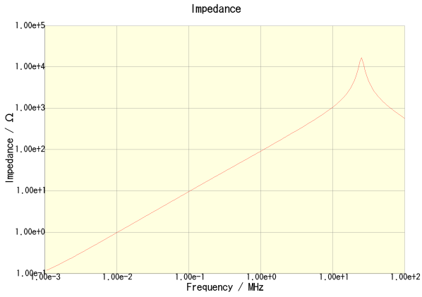
CLF6045T-150M
