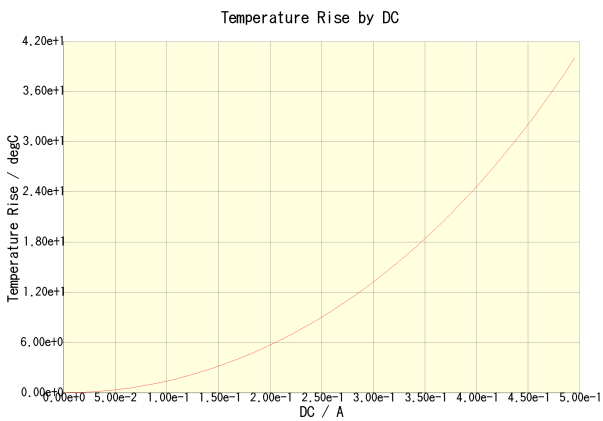
CLF6045T-331M(Amb. Temp. = 20degc)
