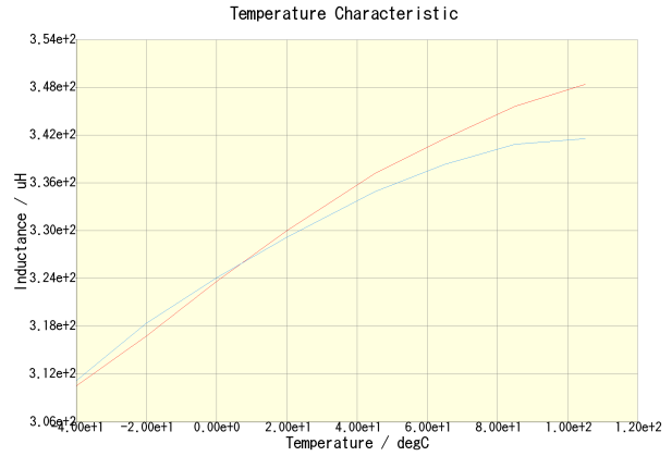
CLF6045T-331M(DC = 0A)
