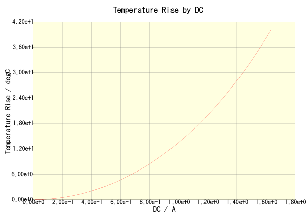
CLF7045T-470M(Amb. Temp. = 20degc)
