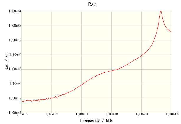
CLF7045T-6R8N
