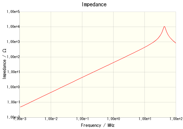
CLF7045T-6R8N
