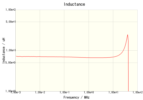
CLF7045T-6R8N
