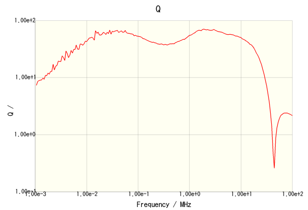
CLF7045T-6R8N
