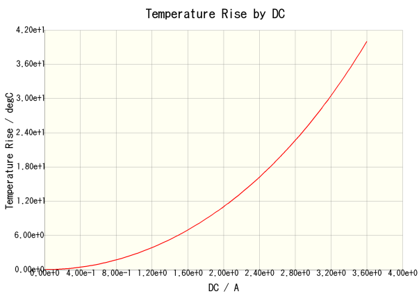
CLF7045T-6R8N(Amb. Temp. = 20degc)
