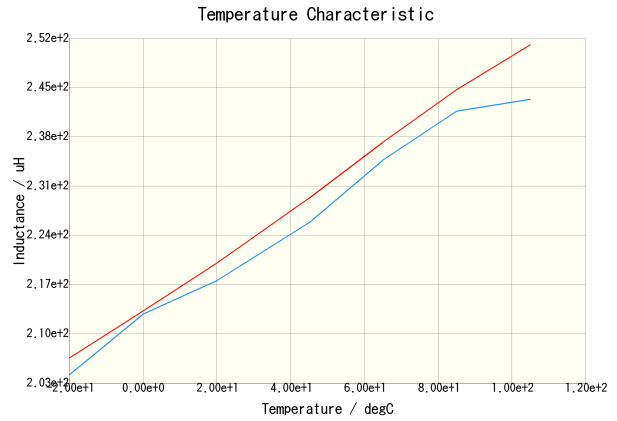
VLCF5028T-221MR22-2(DC = 0A) VLCF5028T-221MR22-2(DC = 0.11A)
