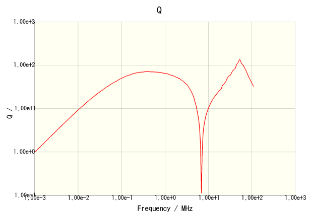
VLCF5028T-221MR22-2
