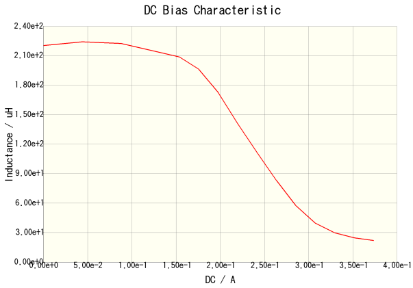
VLCF5028T-221MR22-2(Amb. Temp. = 20degc)
