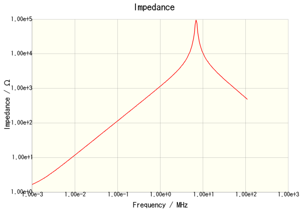
VLCF5028T-221MR22-2
