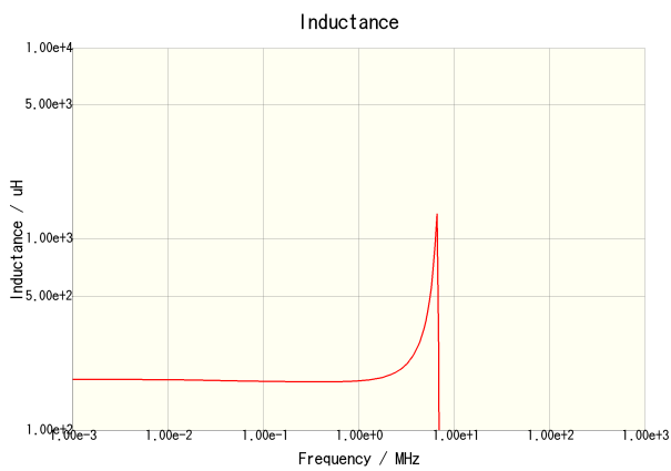
VLCF5028T-221MR22-2
