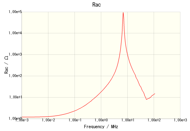
VLCF5028T-221MR22-2
