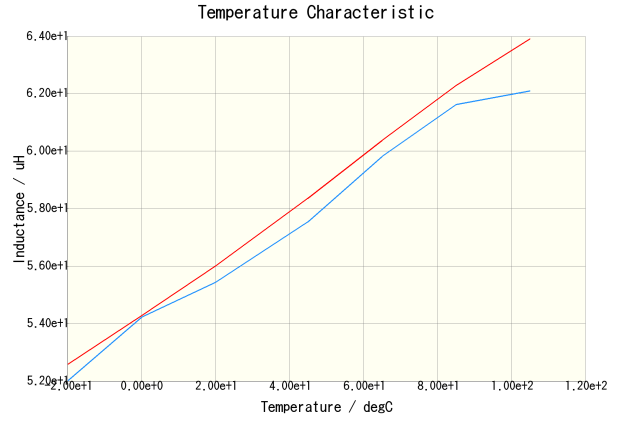
VLCF5028T-560MR43-2(DC = 0A) VLCF5028T-560MR43-2(DC = 0.215A)
