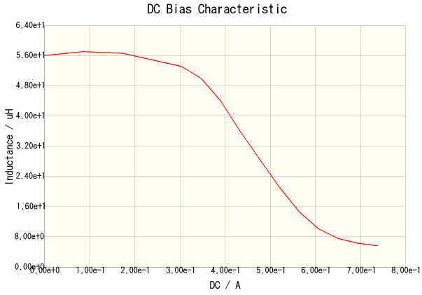
VLCF5028T-560MR43-2(Amb. Temp. = 20degc)
