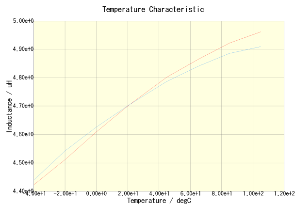
CLF6045T-4R7N(DC = 0A)
