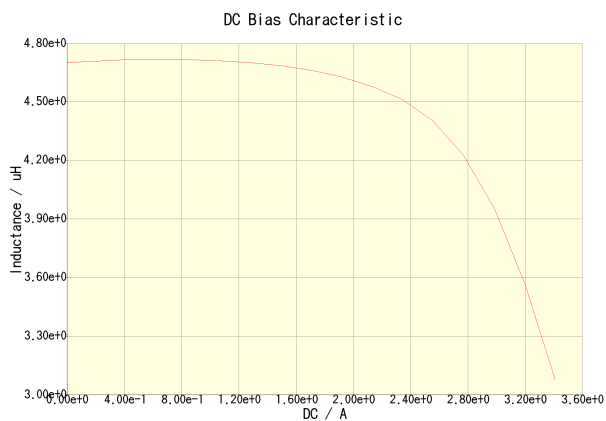
CLF6045T-4R7N(Amb. Temp. = 20degc)
