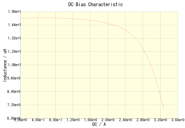
CLF7045T-150M(Amb. Temp. = 20degc)
