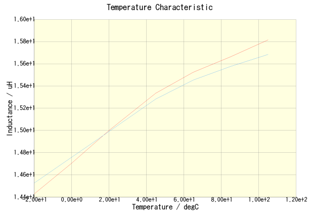
CLF7045T-150M(DC = 0A)
