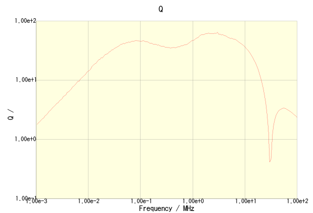
CLF7045T-150M
