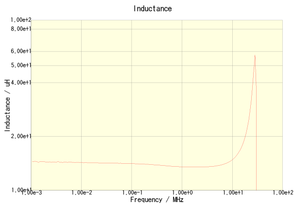
CLF7045T-150M
